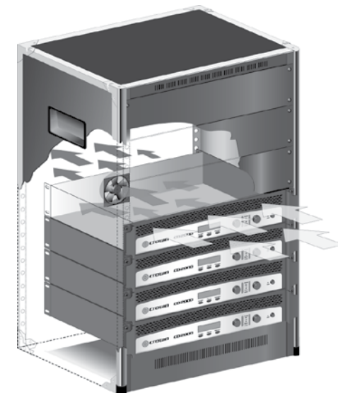
Figure 2.2 Airflow
